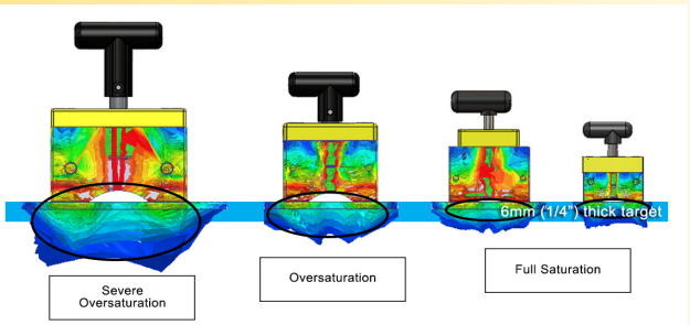
Airgap Performance (1/4in (6mm) thick target)
