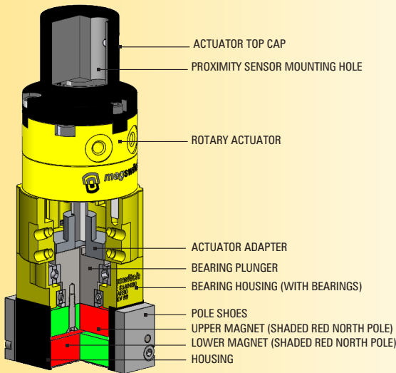
MAGSWITCH CUTAWAY – OFF POSITION
